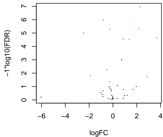
Volcano plot
