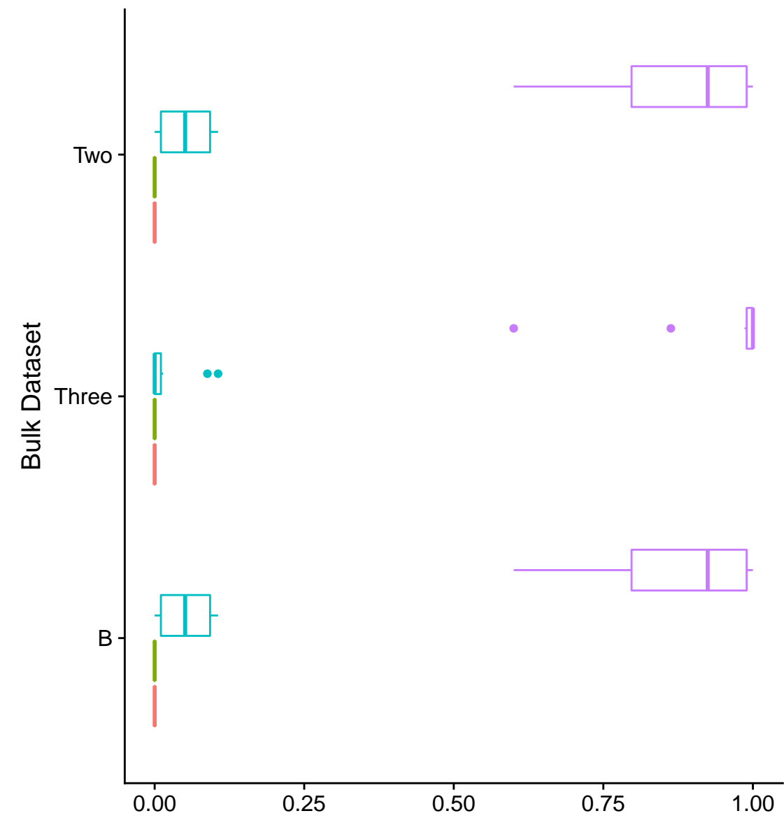
Sample
