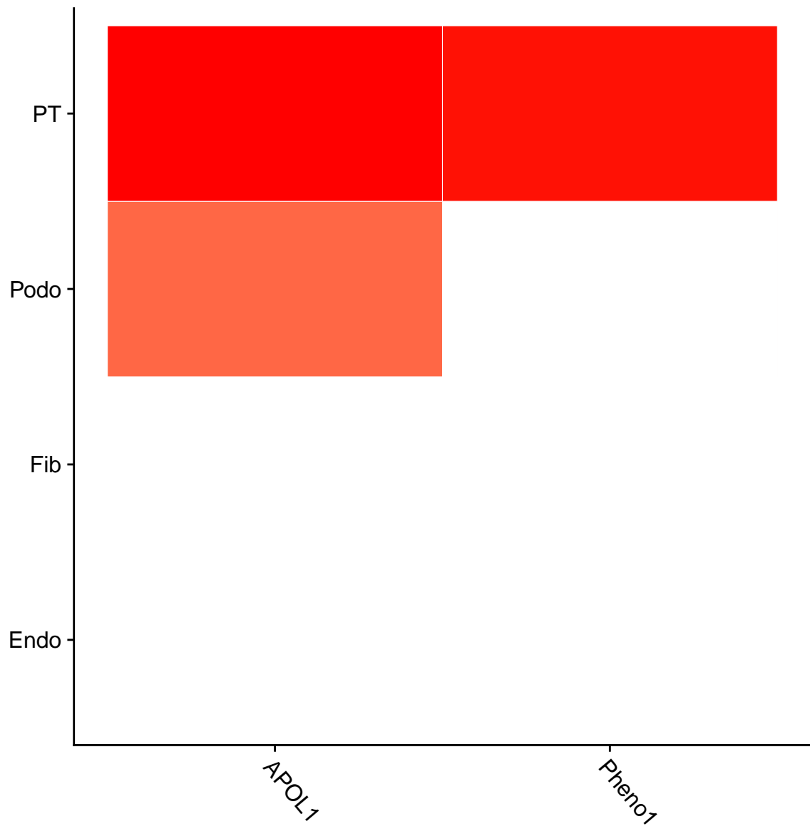
Reads (log10+1)
