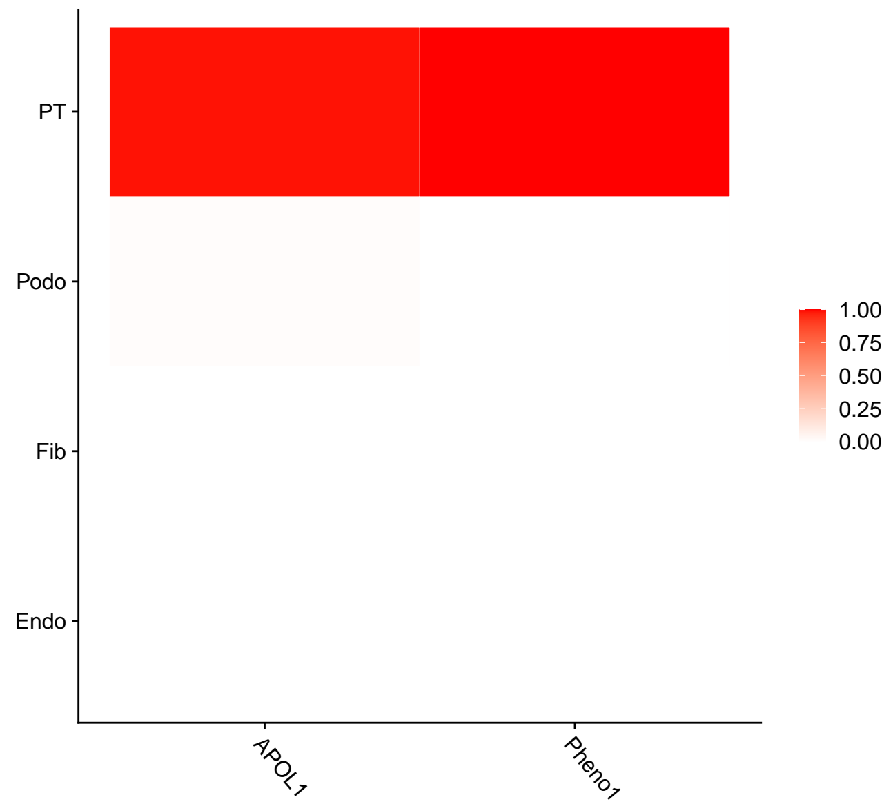
Sample
