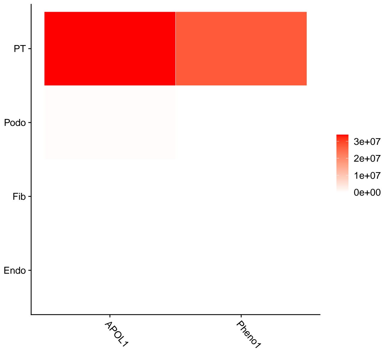
Reads
