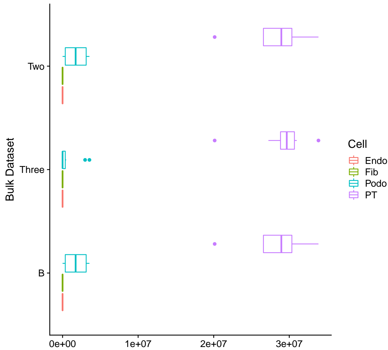
Reads
