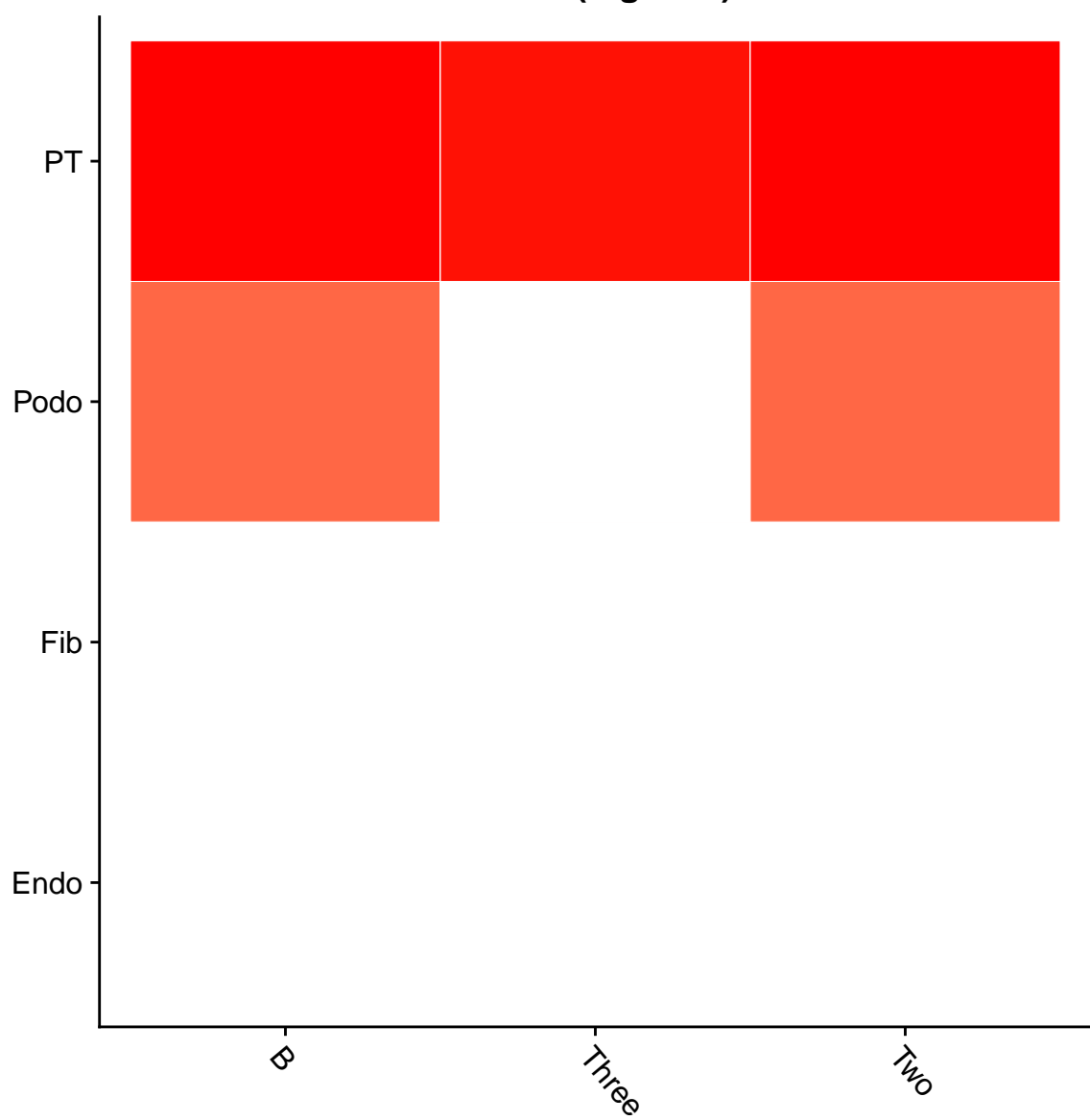
Reads (log10+1)
