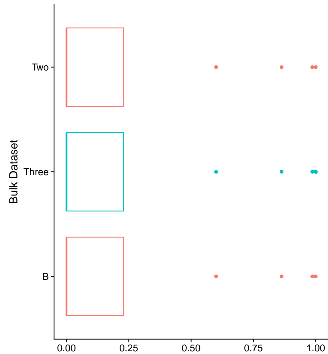
Sample
