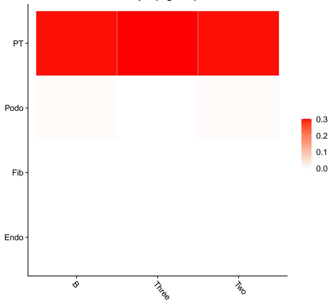
Sample (log10+1)
